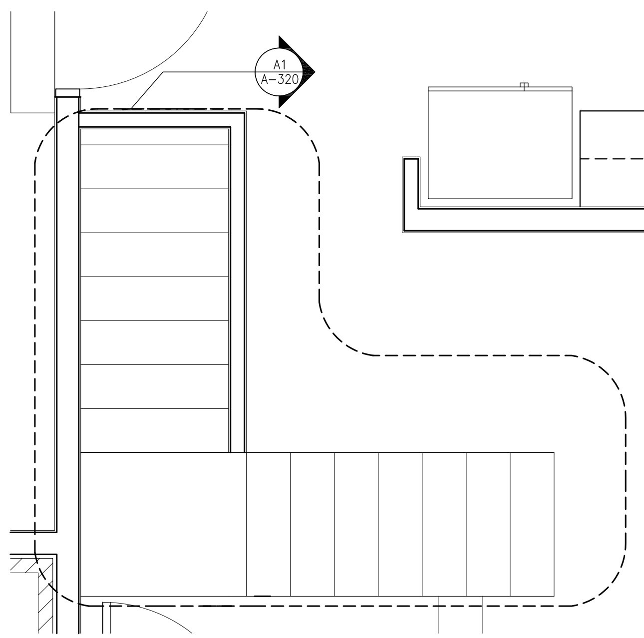
STAIR PLAN 'A' FIRST FLOOR SCALE 1/2"=1'-0" A1
