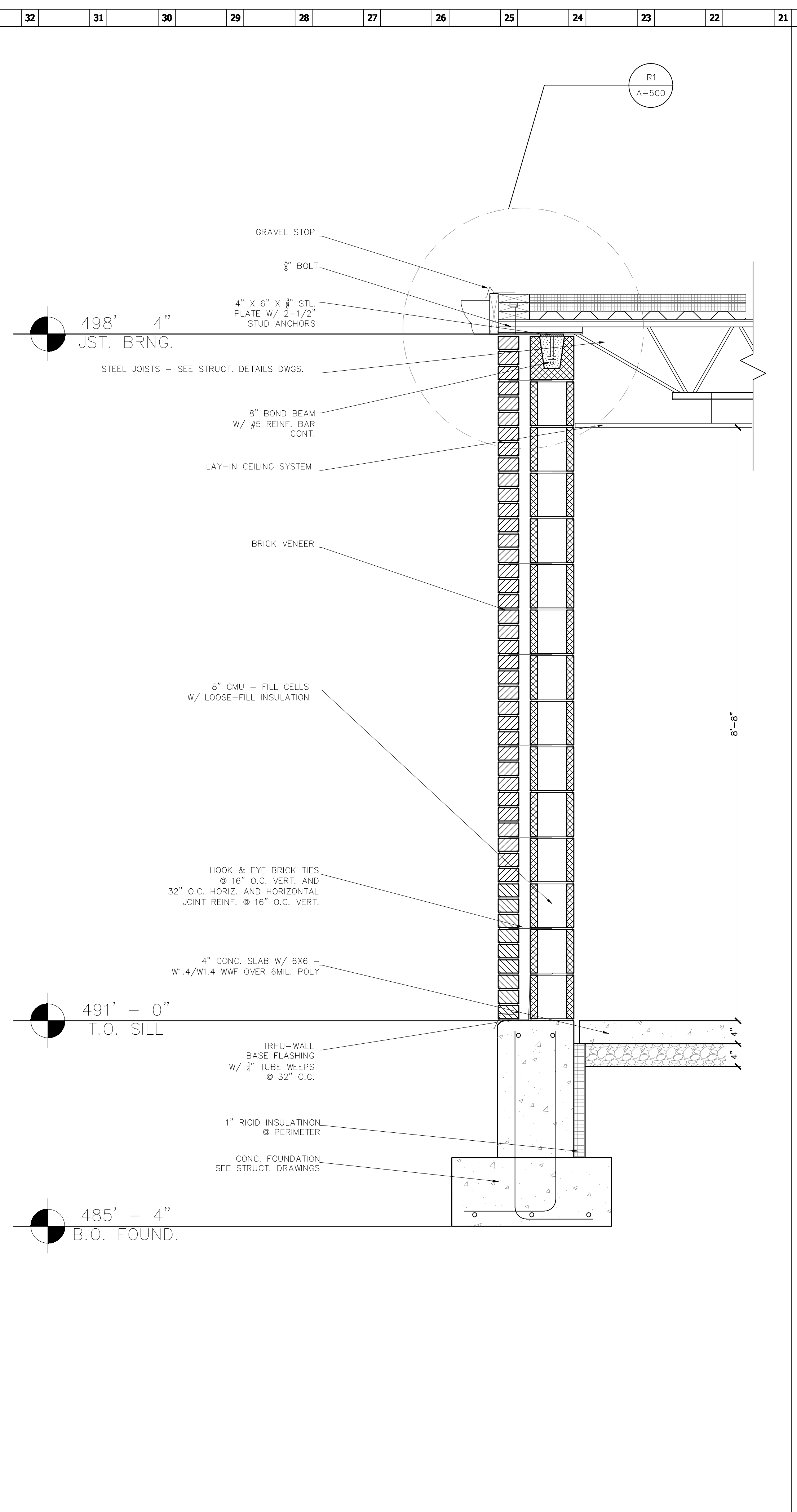
WALL SECTION W/O WINDOW SCALE 1/4"=1'-0" A21
