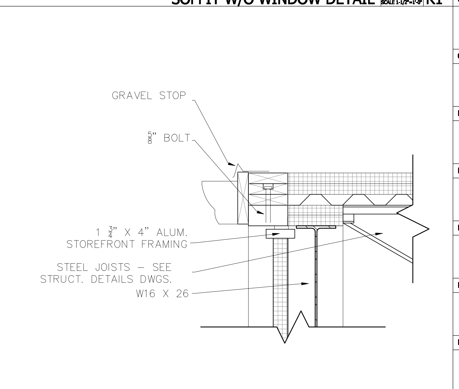
SOFFIT W/ WINDOW DETAIL SCALE 1/2"=1'-0" J1
