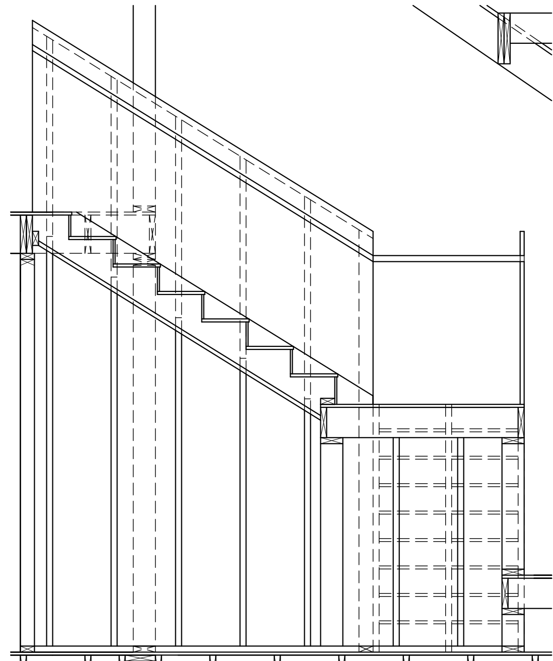
STAIR SECTION SCALE 1/2"=1'-0" H8
