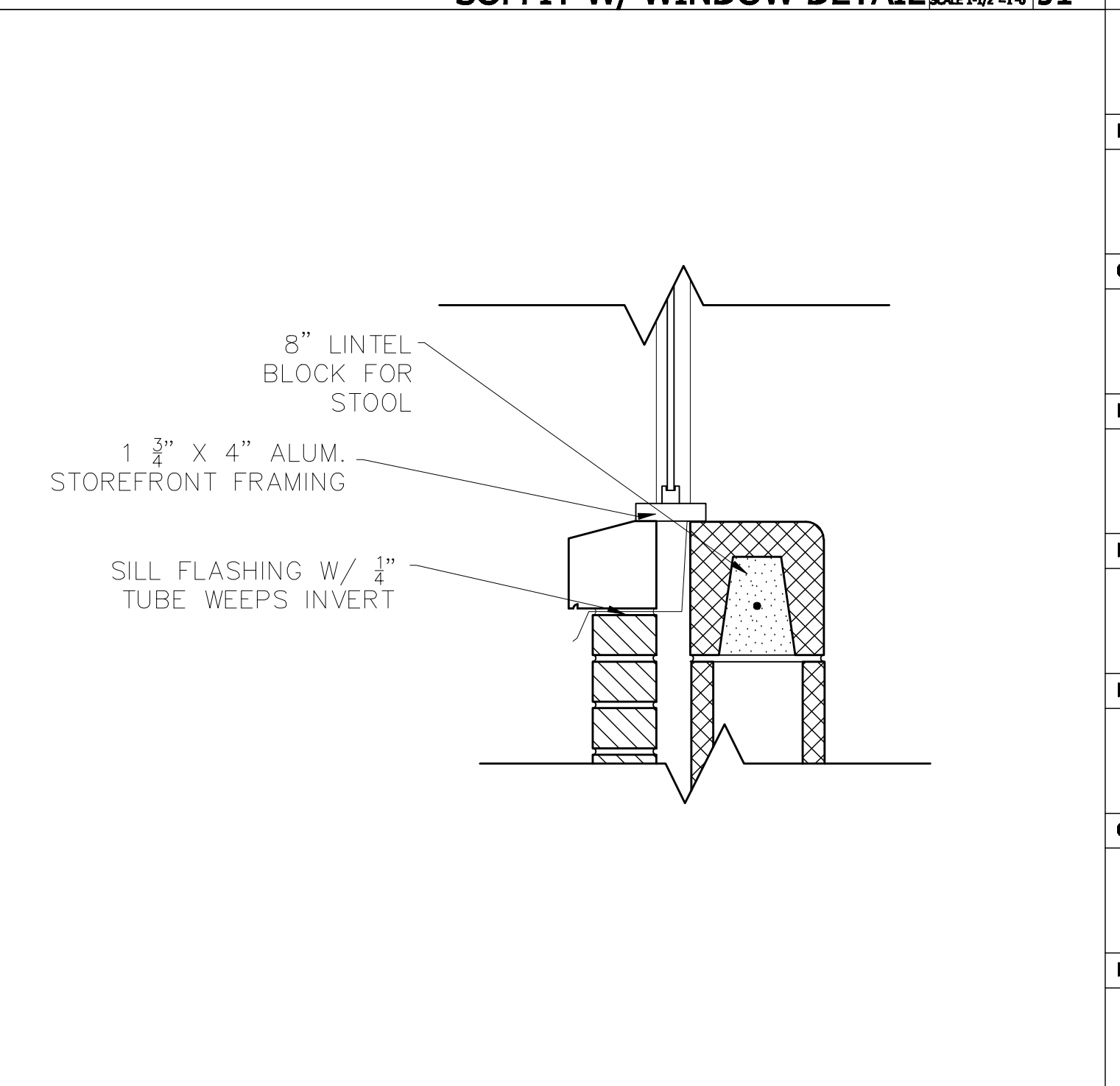
WINDOW SILL DETAIL SCALE 1/2"=1'-0" A1
