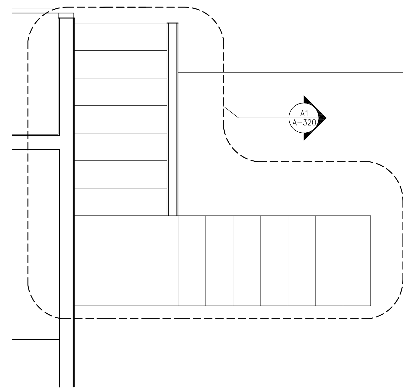
STAIR PLAN 'B' SECOND FLOOR SCALE 1/2"=1'-0" H1
