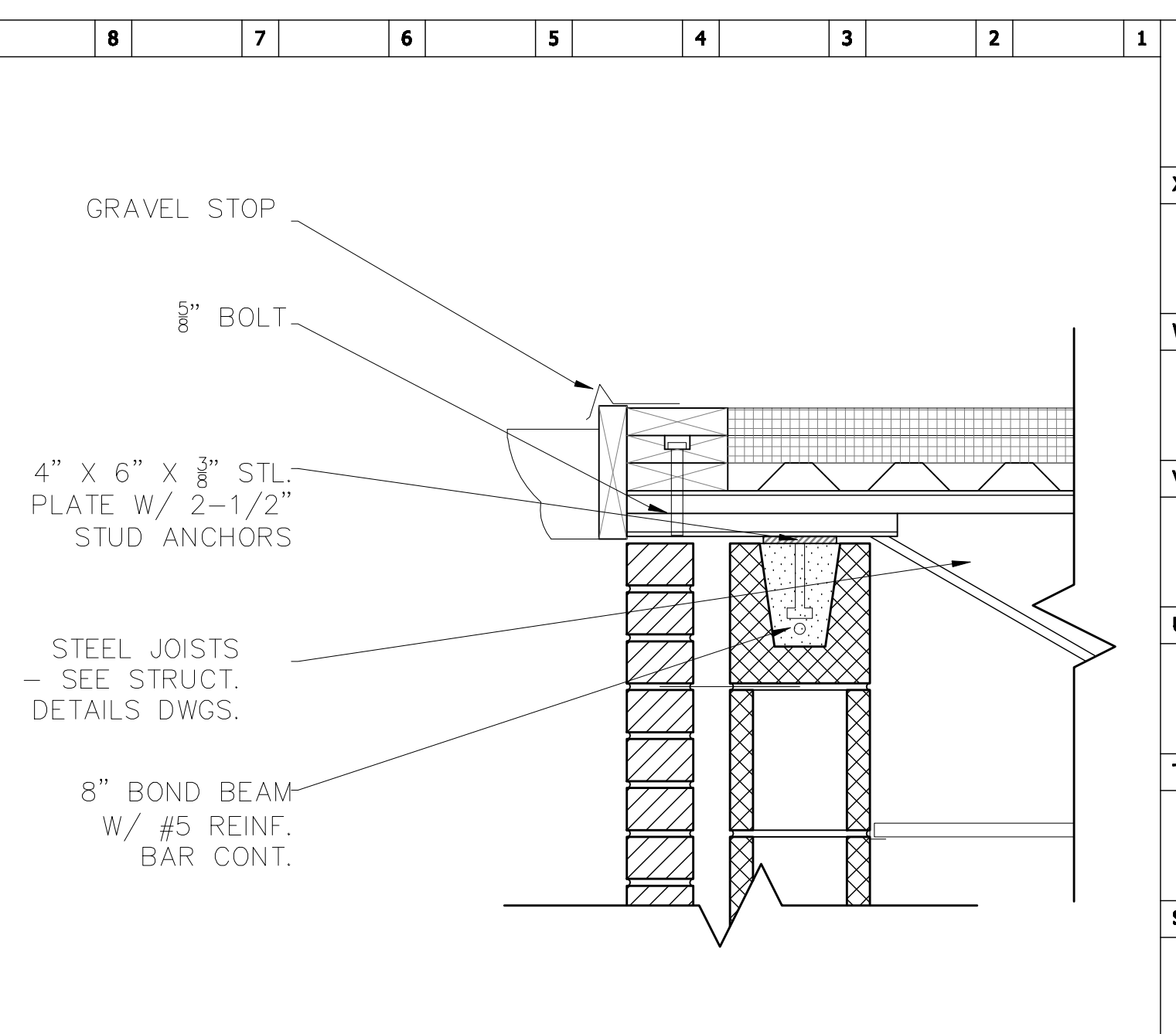
SOFFIT W/O WINDOW DETAIL SCALE 1/2"=1'-0" R1
