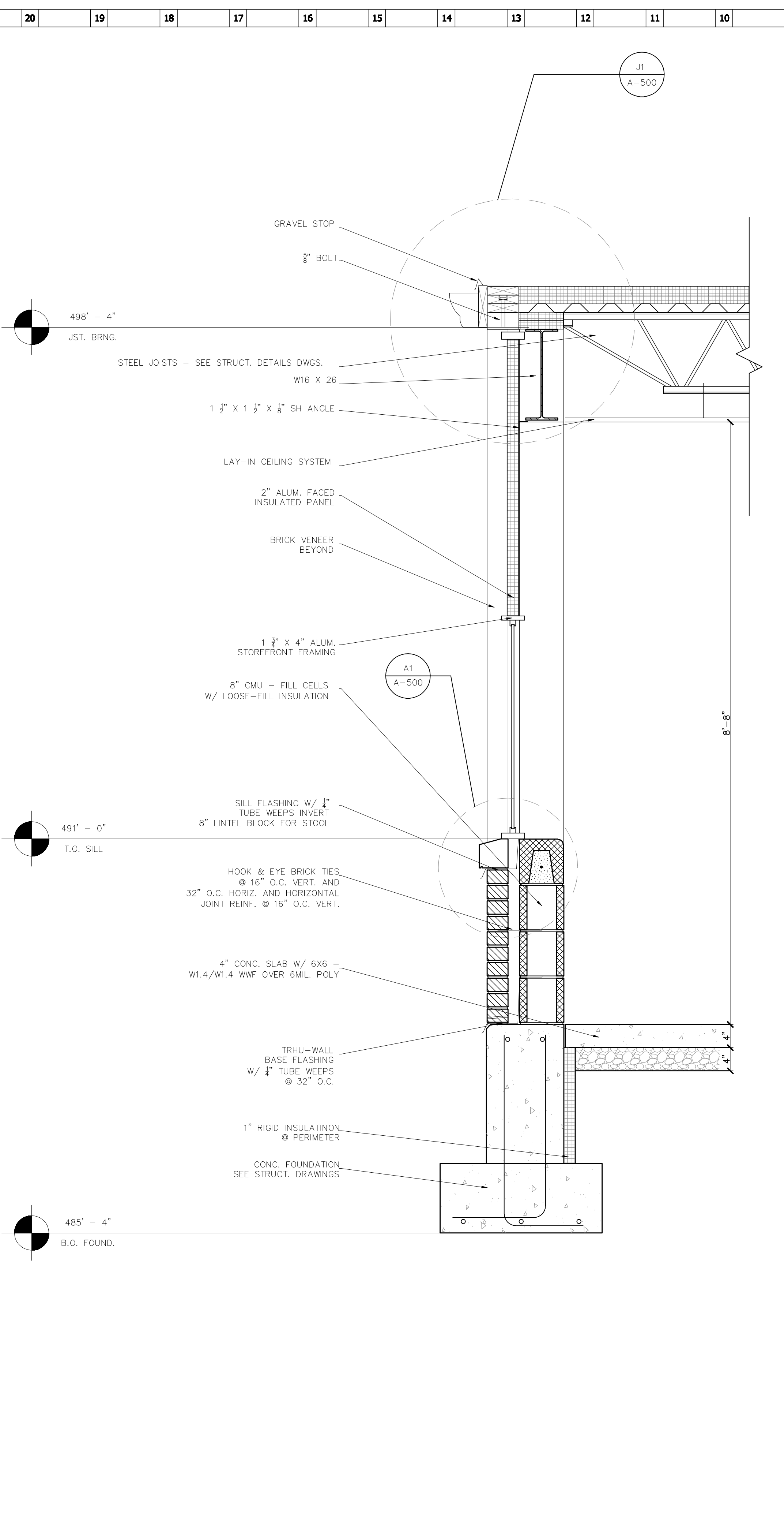
WALL SECTION W/ WINDOW SCALE 1/4"=1'-0" A9
